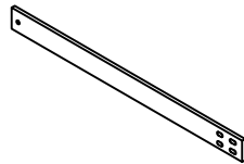
Center Support Front Rail 48-3/4" x 3-9/16" x 13/16"
